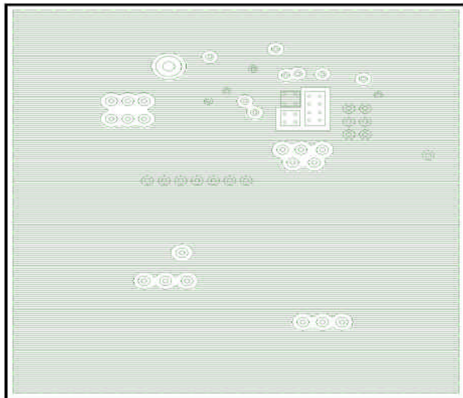
Figure 16 Ground layer
